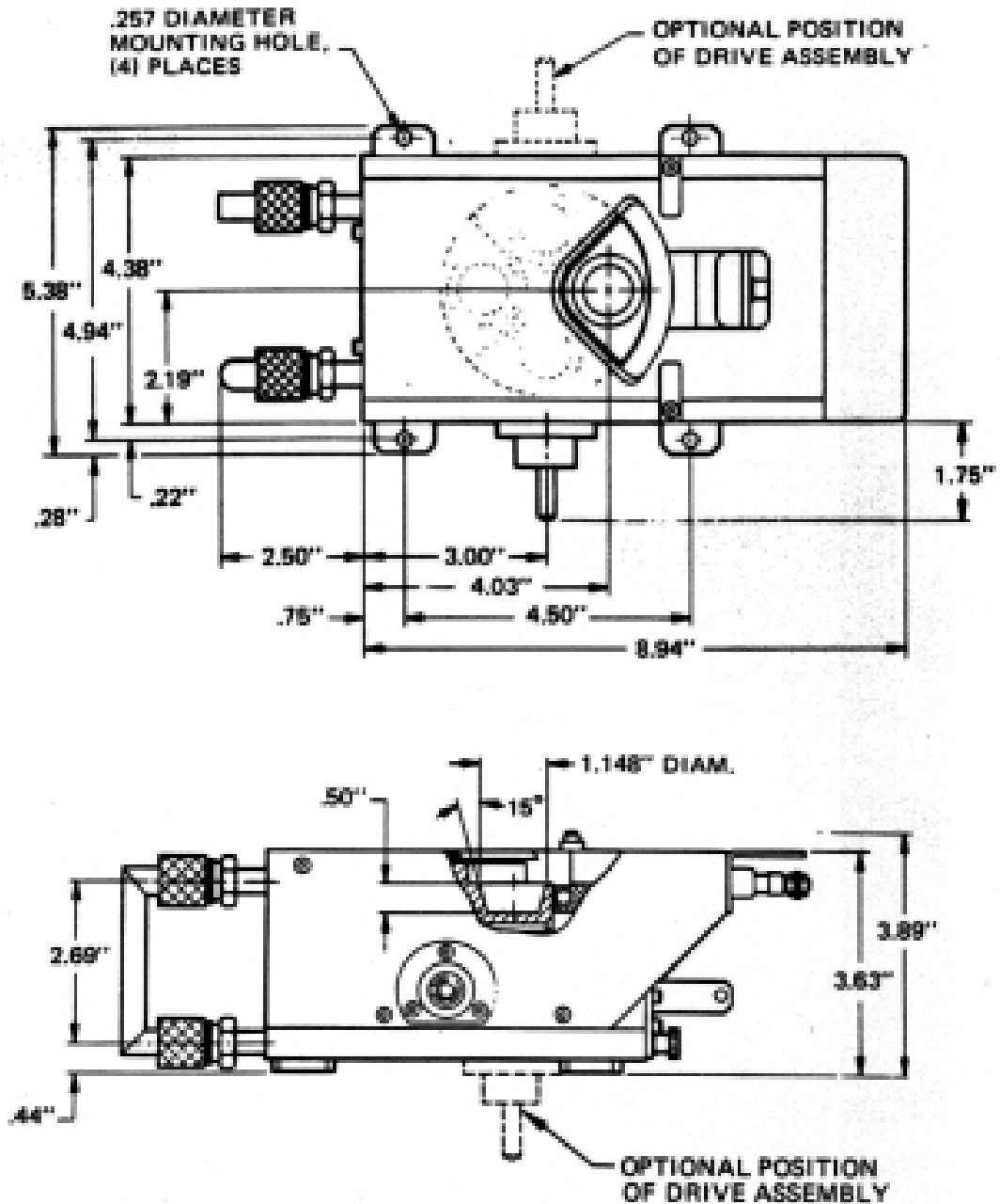
Figure 1. Model STIH-270-1 dimensional drawing
